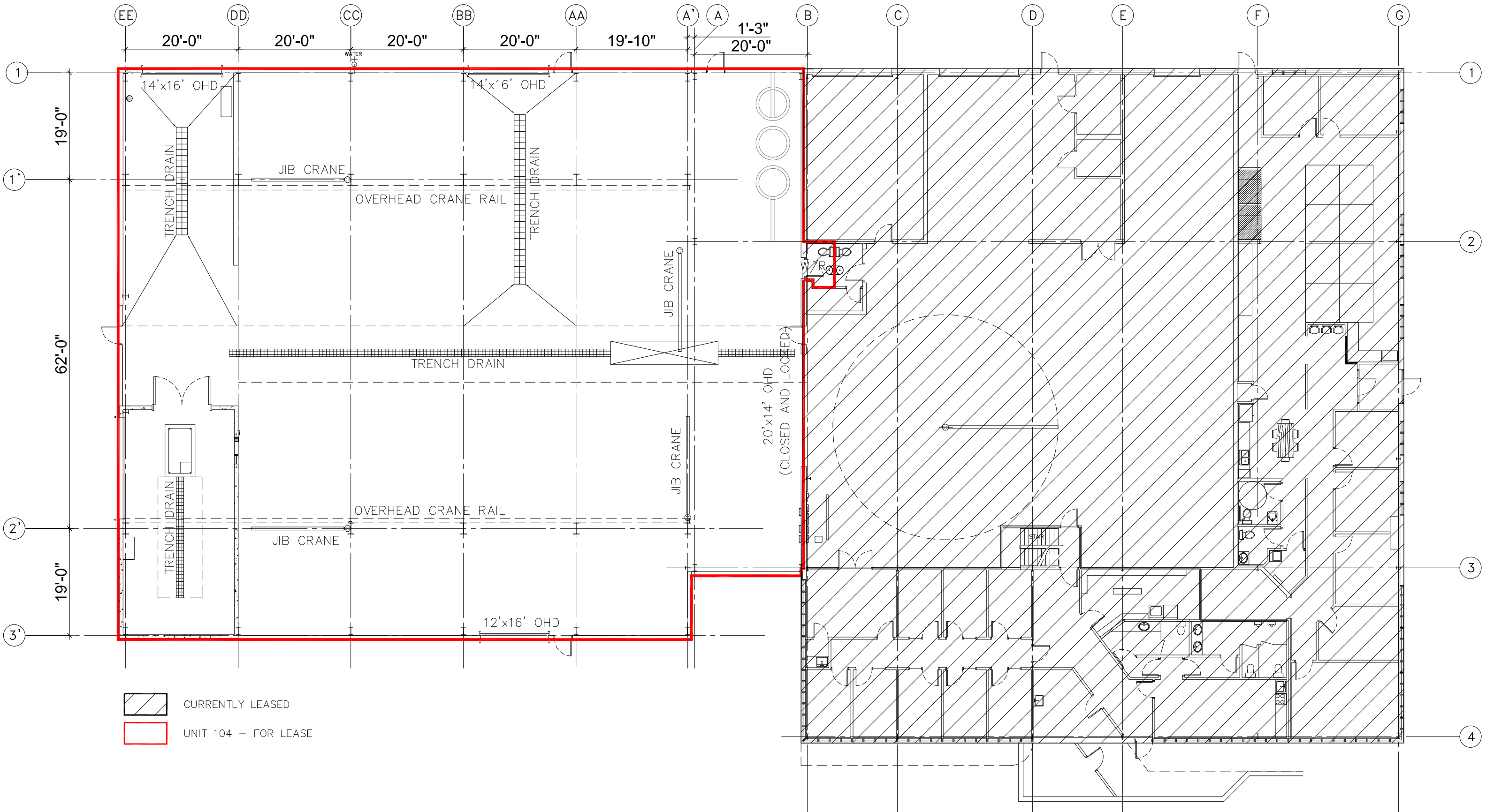
GROUND FLOOR PLAN SCALE 1/16" = 1'-0"
